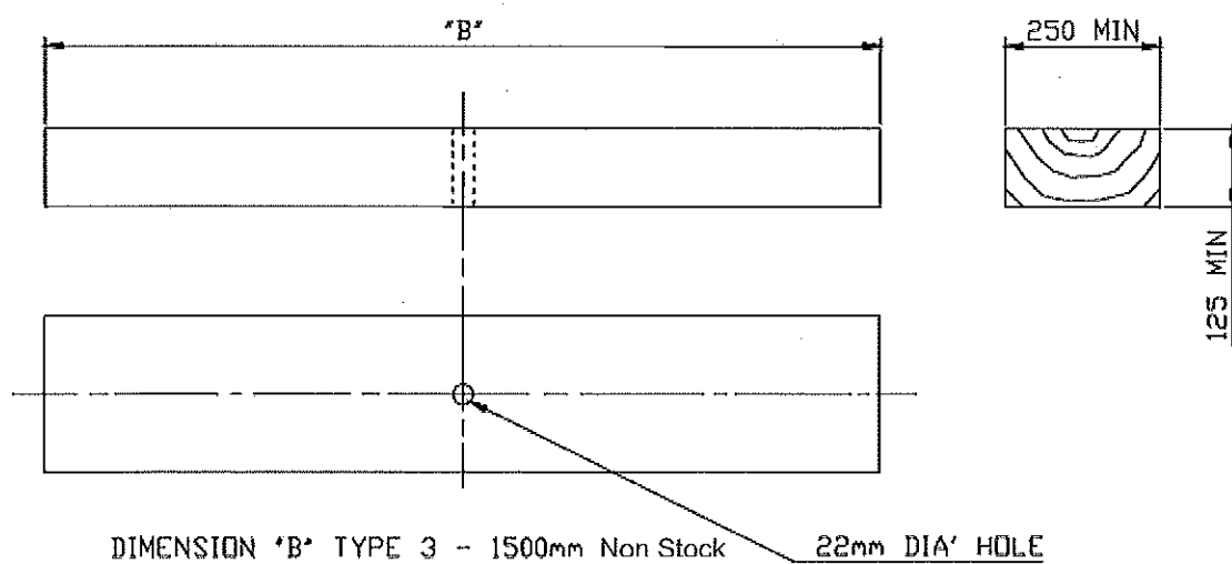
Fig. 439103 - Wood Stay and Foundation Blocks
